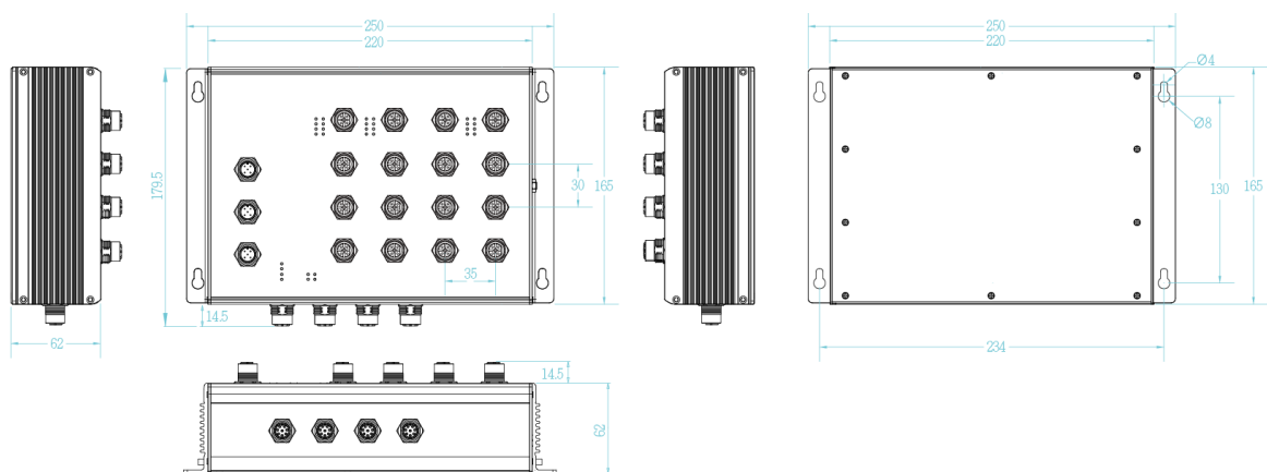
IP54 model
