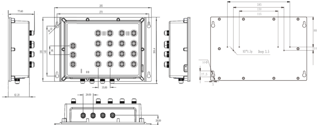
IP54 model
